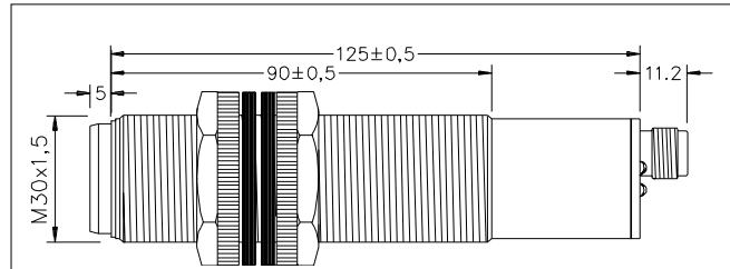
Dimensions/Abmessungen/Dimensions
