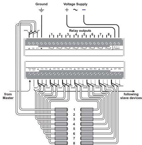
picture 2: Wiring diagram
