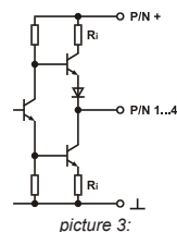
picture 3: transistor output
