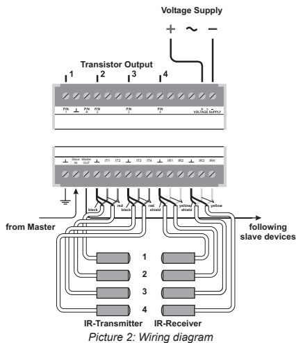
Picture 2: Wiring diagram
